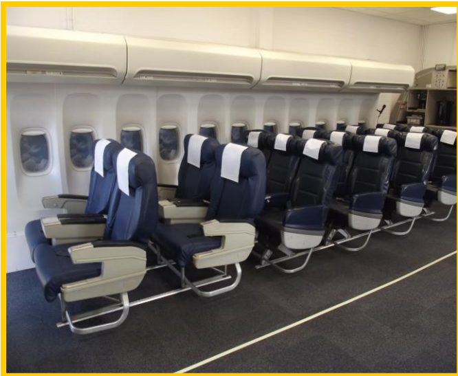
Larger Half Mock-up Two Class Cabin + Check-in Set-up with Security Arch
